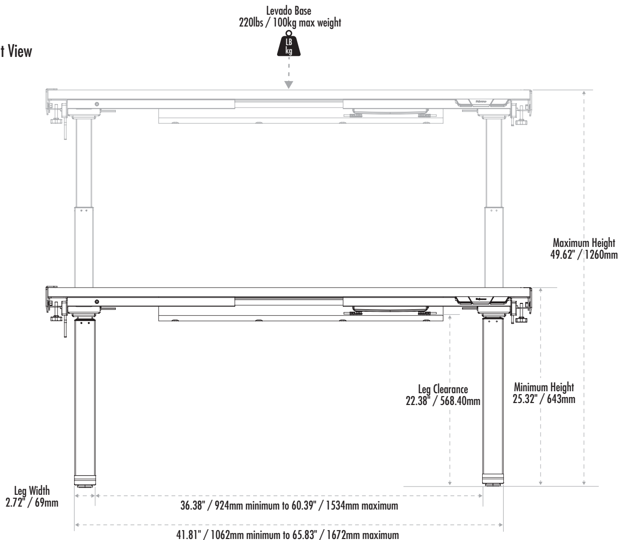
Side View
